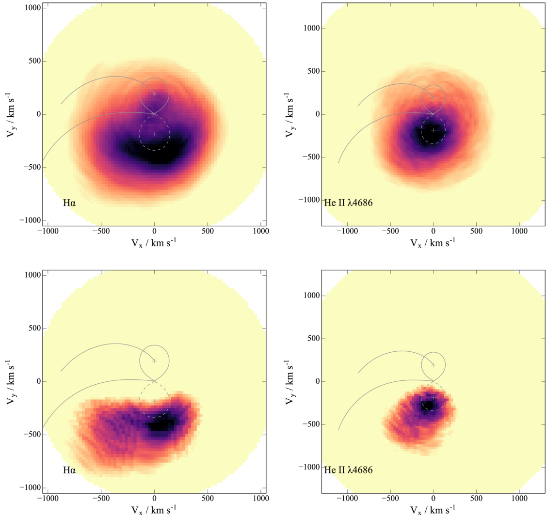
Figure 10. Doppler tomography of J0644 for (left) H\alpha and (right) He\ II\ \lambda 4686 -Å emission lines. The Roche lobe surface was calculated using the orbital parameters discussed in this article: i = 78^\circ , q = 0.96 and \gamma = -7.1\text{ km s}^{-1} . The Keplerian and ballistic trajectories in the upper figures are marked as the upper and lower curves, respectively. The crosses are the velocity (from top to bottom) of the secondary star, the centre of mass and the primary star. (See text for discussion.) The bottom figures show the same tomograms after subtracting an azimuthal average to highlight the asymmetric emission components.
